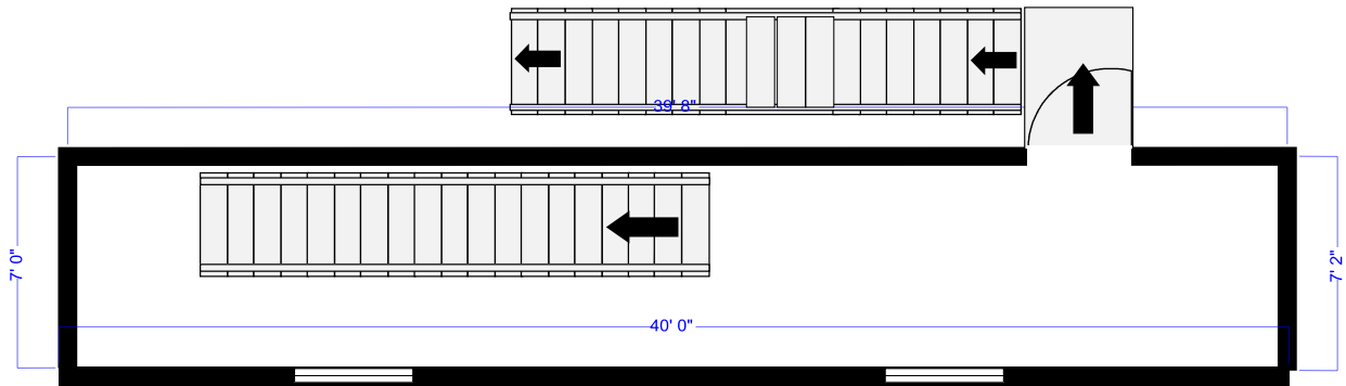
FORT NELSON FIRE RESCUE BURN BUILDING - FIRST FLOOR PLAN
