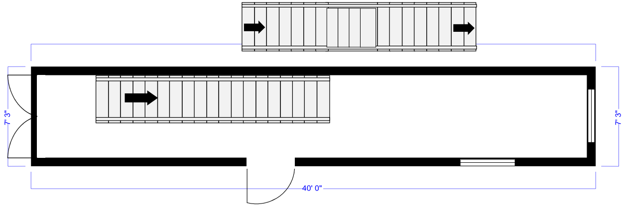
FORT NELSON FIRE RESCUE BURN BUILDING - GROUND FLOOR PLAN
